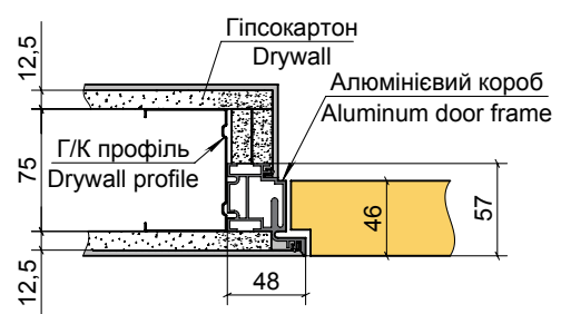
Aluminum door frame iDoors "INSIDE" reverse opening
