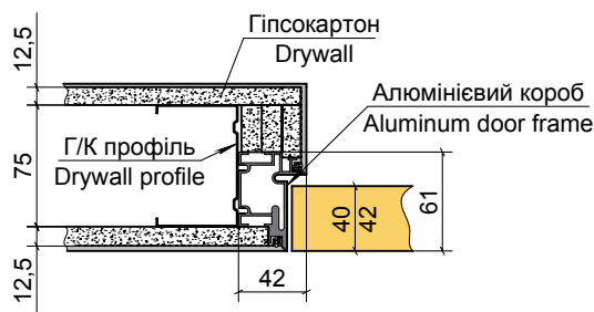
Aluminum door frame iDoors "Standard" external opening
