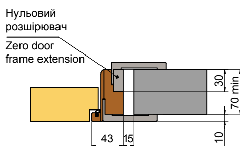
Короб "Компланарний (inside)" Door frame "Coplanar (inside)"
