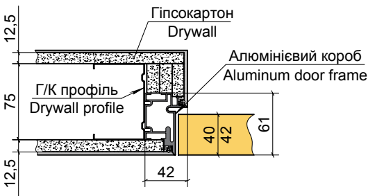
Aluminum door frame iDoors "Standard" external opening
